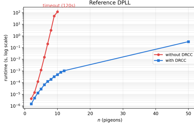
Figure 2: Reference DPLL: runtime without DRCC reaches the 120s timeout ceiling at n = 10 and is not plotted beyond that point; with DRCC it remains solved through n = 50 . The visible DRCC curve exhibits a change in its growth regime; this curve transition is distinguished from the formal runtime crossover defined in Section 3.1.6.
