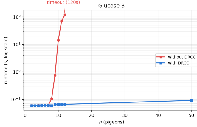
Figure 4: Glucose 3: runtime without DRCC reaches the timeout ceiling at n = 12 ; with DRCC it remains solved through n = 50 . No formal W or W_{\text{int}} is observed because the measured G_{\text{time}}(n) does not fall below unity; its minimum is G_{\text{time}}(3) = 1.003 .
