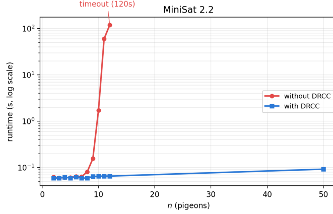
Figure 3: MiniSat 2.2: runtime without DRCC reaches the timeout ceiling at n = 12 ; with DRCC it remains solved through n = 50 . A formal discrete crossover interval W_{\text{int}} = [4, 5] is identified, but both endpoints lie within the subprocess-overhead/noise band and are therefore not interpreted as the practically relevant onset.
