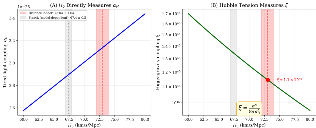
Figure 5: (A) : The tired light coupling \alpha_H as a function of the measured photon fade rate H_0 = c/\lambda_H . The distance ladder measurement (red band) directly determines \alpha_H ; the Planck value (gray band) is model-dependent and invalid in this framework. (B) : The Higgs-gravity coupling \xi derived from H_0 via \xi = \alpha^4/(8\pi\alpha_H^2) . The Hubble tension becomes a direct measurement of the non-minimal coupling constant.
