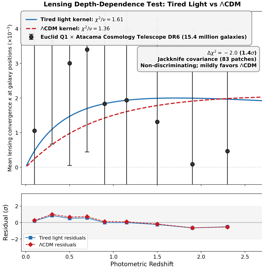
Figure 13: Euclid Q1 × Atacama Cosmology Telescope DR6 depth dependence test. Mean lensing convergence \langle\kappa\rangle in 9 redshift bins (black points with calibrated pixel-level error bars) compared to the tired light prediction (blue curve) and \Lambda CDM prediction (red curve). With a proper jackknife covariance the two kernels are statistically indistinguishable over this range ( \Delta\chi^2 \approx -2 , 1.4\sigma , mildly favoring \Lambda CDM). The signal peaks at z \approx 0.3 – 0.7 and declines monotonically, a shape consistent with both kernels below z = 2.5 .
