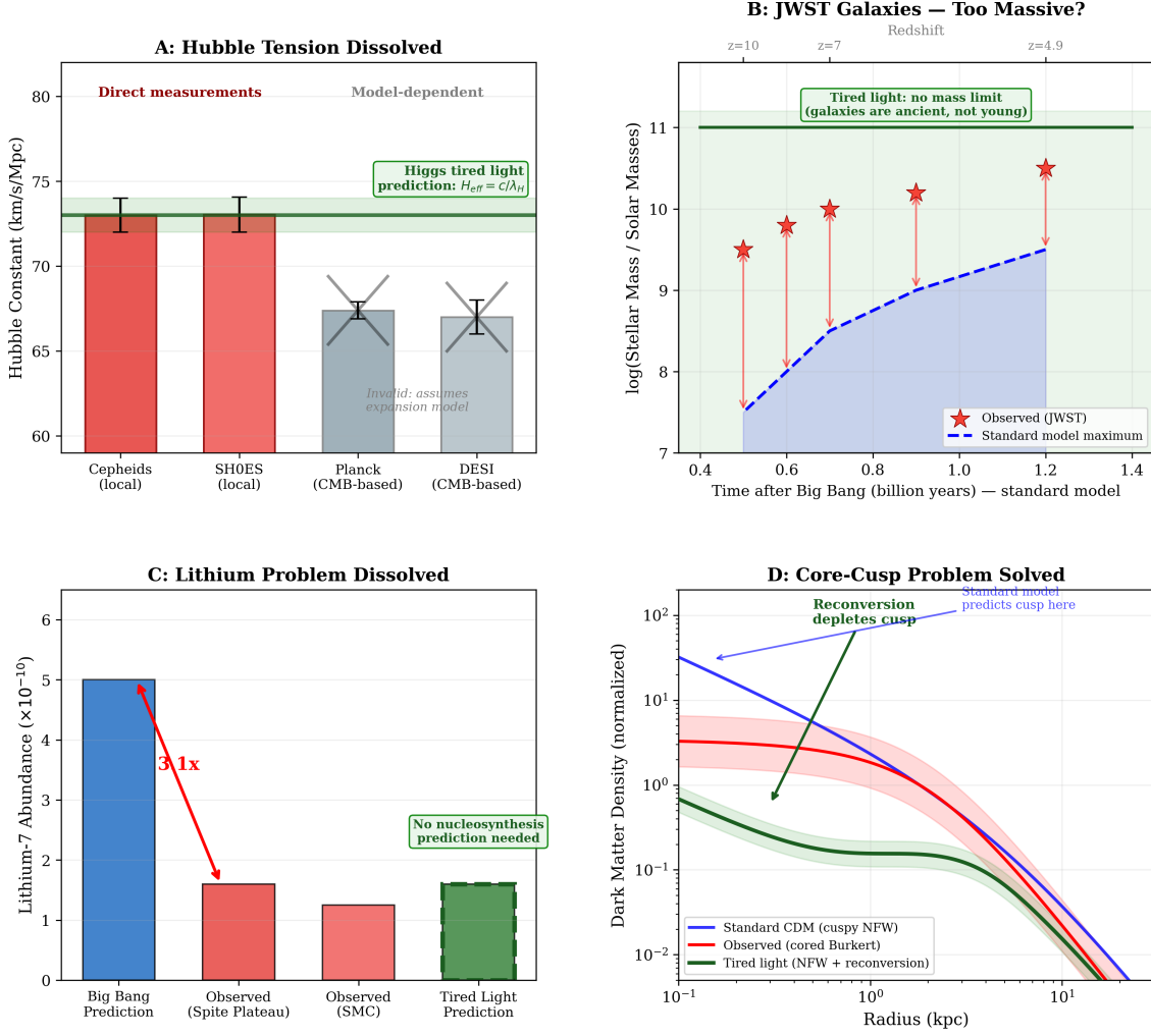
Figure 15: Observational evidence supporting tired light cosmology. Green elements show our framework’s predictions. (A) : Hubble tension— >5\sigma disagreement between measurement methods; our effective H_0 = c/\lambda_H avoids the tension entirely. (B) : James Webb Space Telescope early galaxies—mature objects at high redshift; no mass limit in a non-expanding universe. (C) : Lithium problem—observed abundance versus Big Bang prediction; no nucleosynthesis prediction needed in our framework. (D) : Core-cusp problem—observed cored profiles versus simulated cusps; reconversion-depleted profiles naturally produce cores.
