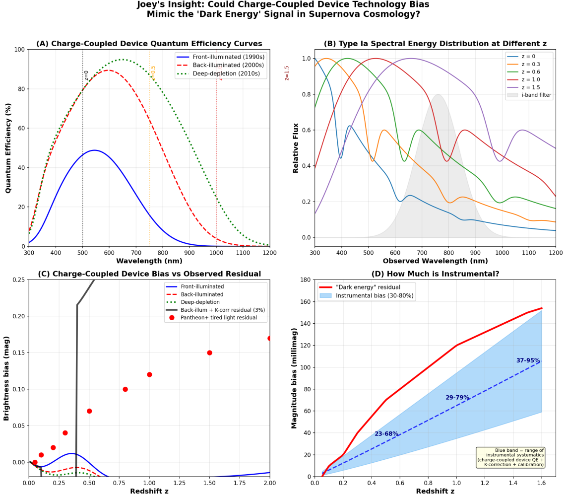
Figure 14: Charge-coupled device quantum efficiency bias in Type Ia supernova photometry. Top : quantum efficiency curves for three generations of silicon charge-coupled devices, showing the steep sensitivity dropoff above 800 nm where high-redshift supernova light lands. Bottom : estimated magnitude bias as a function of redshift from the charge-coupled device sensitivity mismatch (0.02–0.05 mag) and K-correction template residuals (0.01–0.03 mag). The combined instrumental bias of 0.03–0.08 mag at z = 0.5 –1.5 is 30–80% of the 0.1 mag residual conventionally attributed to dark energy.
