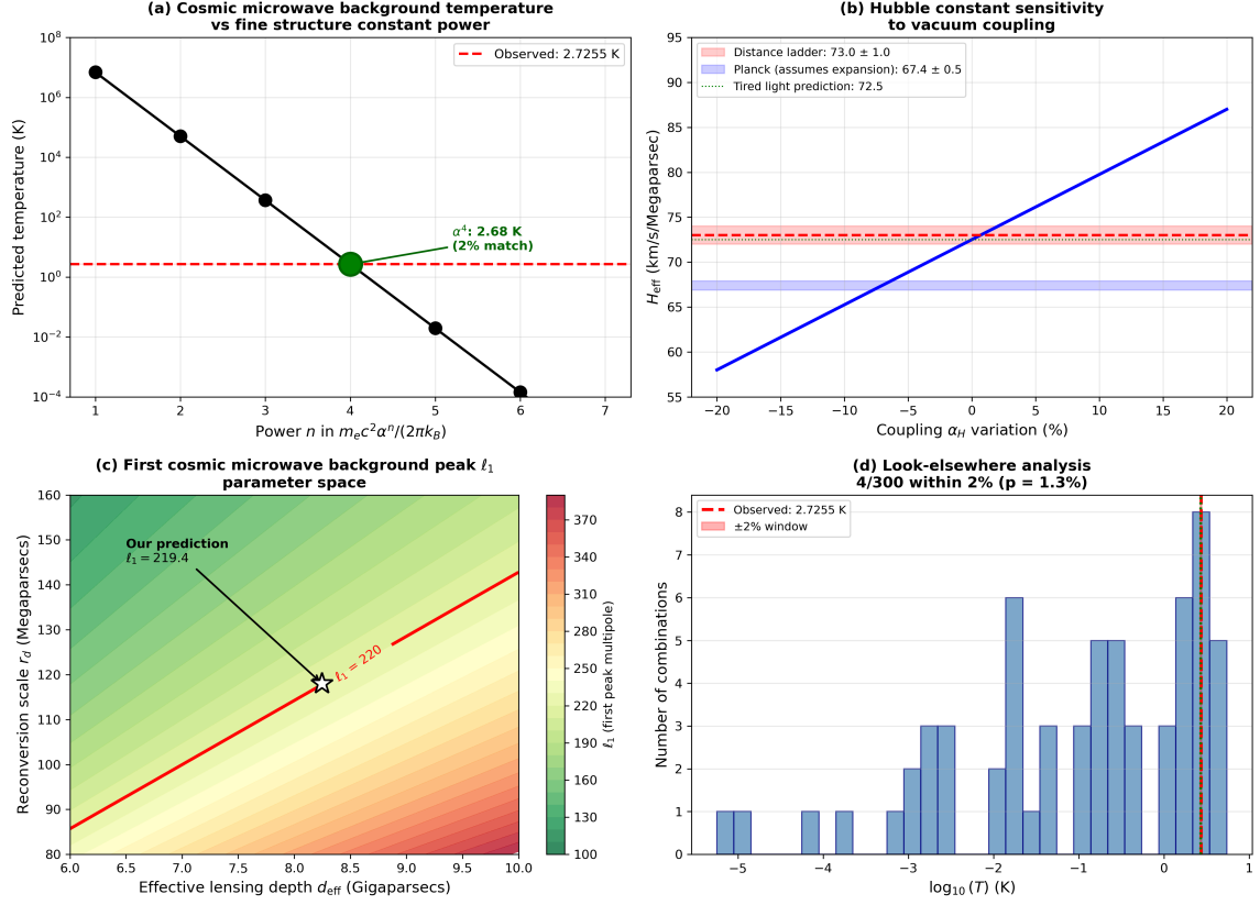
Figure 24: Sensitivity analysis of key predictions. (a) Cosmic microwave background temperature vs. fine structure constant power: only \alpha^4 matches (1.8%); adjacent powers miss by factor 137. (b) Hubble constant sensitivity to vacuum coupling variation. (c) First peak \ell_1 parameter space over effective depth and reconversion scale; our prediction (star) lies on the \ell_1 = 220 contour. (d) Look-elsewhere analysis: 4/300 combinations match T_{\text{obs}} within 2% ( p = 1.3\% ).
