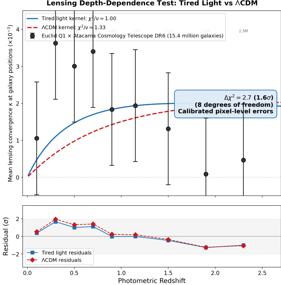
Figure 17: Euclid Q1 \times Atacama Cosmology Telescope DR6 depth dependence test. Mean lensing convergence \langle\kappa\rangle in 9 redshift bins (black points with calibrated pixel-level error bars) compared to the tired light prediction (blue curve) and \Lambda CDM prediction (red curve). The tired light kernel provides a better fit ( \Delta\chi^2 = 2.65 , 1.6\sigma ). The signal peaks at z \approx 0.3\text{--}0.7 and declines monotonically, consistent with the tired light kernel shape.
