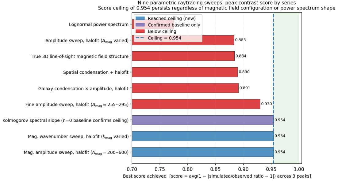
Figure 8: Summary of nine parametric raytracing sweeps. The score axis measures average accuracy across three peak contrast ratios: \text{score} = \frac{1}{3} \sum_{i=1}^3 (1 - |r_i^{\text{sim}}/r_i^{\text{Planck}} - 1|) , where a perfect match gives 1.0. Blue bars: configurations that independently reached the ceiling of 0.954. Purple bar: the Kolmogorov slope sweep, which confirmed the ceiling only because the zero-slope baseline is identical to the best amplitude configuration — every non-zero slope performed worse. Red bars: all other parametric variations, all of which fell below 0.954. The ceiling is structural: it arises from 2D projection geometry, not from any physical parameter being suboptimal.
