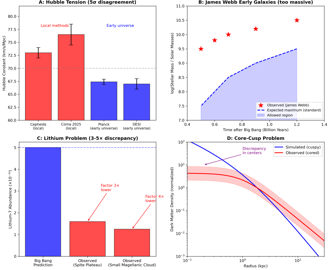
Figure 14: Observational evidence supporting tired light cosmology. Green elements show our framework’s predictions. (A) : Hubble tension— >5\sigma disagreement between measurement methods; our effective H_0 = c/\lambda_H avoids the tension entirely. (B) : James Webb Space Telescope early galaxies—mature objects at high redshift; no mass limit in a non-expanding universe. (C) : Lithium problem—observed abundance versus Big Bang prediction; no nucleosynthesis prediction needed in our framework. (D) : Core-cusp problem—observed cored profiles versus simulated cusps; reconversion-depleted profiles naturally produce cores.
