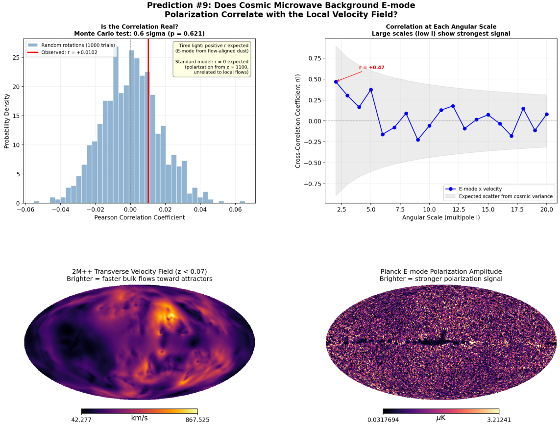
Figure 17: Prediction #9 test: Planck SMICA E-mode polarization cross-correlated with the 2M++ transverse velocity field ( z < 0.07 ). Upper left: Monte Carlo significance test—the observed correlation r = +0.010 (red line) falls within the random distribution ( 0.6\sigma ), as expected given the shallow depth. The prediction box contrasts tired light (positive r from flow-aligned dust) with \Lambda CDM (zero correlation). Upper right: Cross-correlation coefficient r_\ell per multipole—large angular scales ( \ell = 2\text{--}5 ) show elevated signal up to r_\ell = +0.47 . Lower panels: Sky maps of the transverse velocity field (left) and E-mode polarization amplitude (right).
