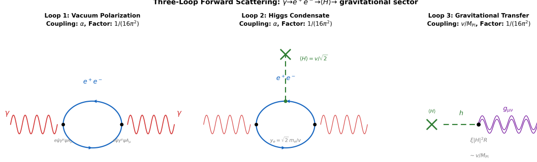
Figure 2: The three loops of the forward scattering process. Loop 1: Standard quantum electrodynamics vacuum polarization ( \gamma \rightarrow e^+ e^- \rightarrow \gamma ), contributing coupling \alpha and loop factor 1/(16\pi^2) . Loop 2: The virtual pair interacts with the Higgs condensate \langle H \rangle = v/\sqrt{2} through the Yukawa coupling, contributing \alpha and 1/(16\pi^2) . Loop 3: Energy transfers to the gravitational sector via the non-minimal coupling \xi |H|^2 R , contributing v/M_{\text{Pl}} and 1/(16\pi^2) .
