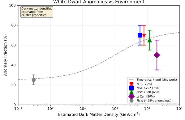
Figure 11: Left: Summary of observed white dwarf anomalies in globular clusters with peer-reviewed references. Right: White dwarf anomaly fraction vs estimated dark matter density, showing real observations (colored points with error bars) and theoretical trend (dashed line).
